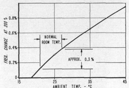
Fig. 5. Stability of typical 200AB with respect to ambient temperature.
