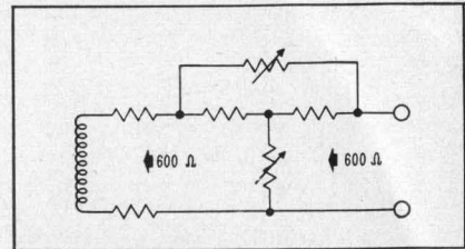
Fig. 7. Basic output circuit of -hp- 200CD.
