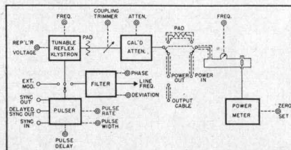
Fig. 1. Circuit block diagram of -hp- Model 624.
